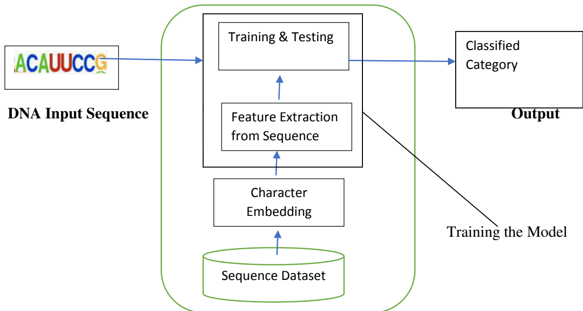
Figure 1: Architecture of DNA/Gene classification System
