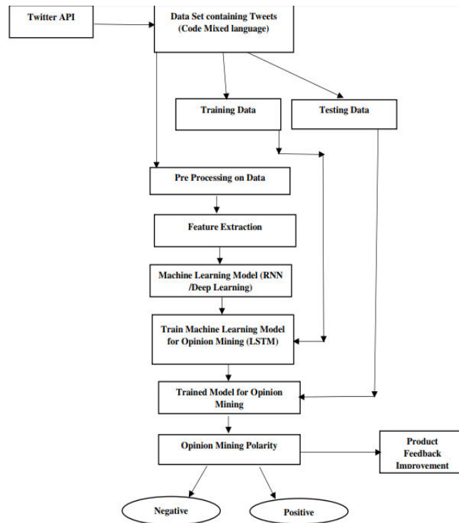
Figure.2 Shows The Flow Chart of Opinion Mining Based on Twitter
